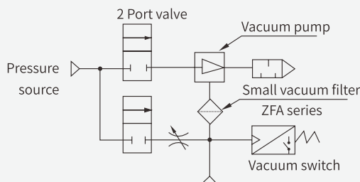
Application of vacuum pump system
